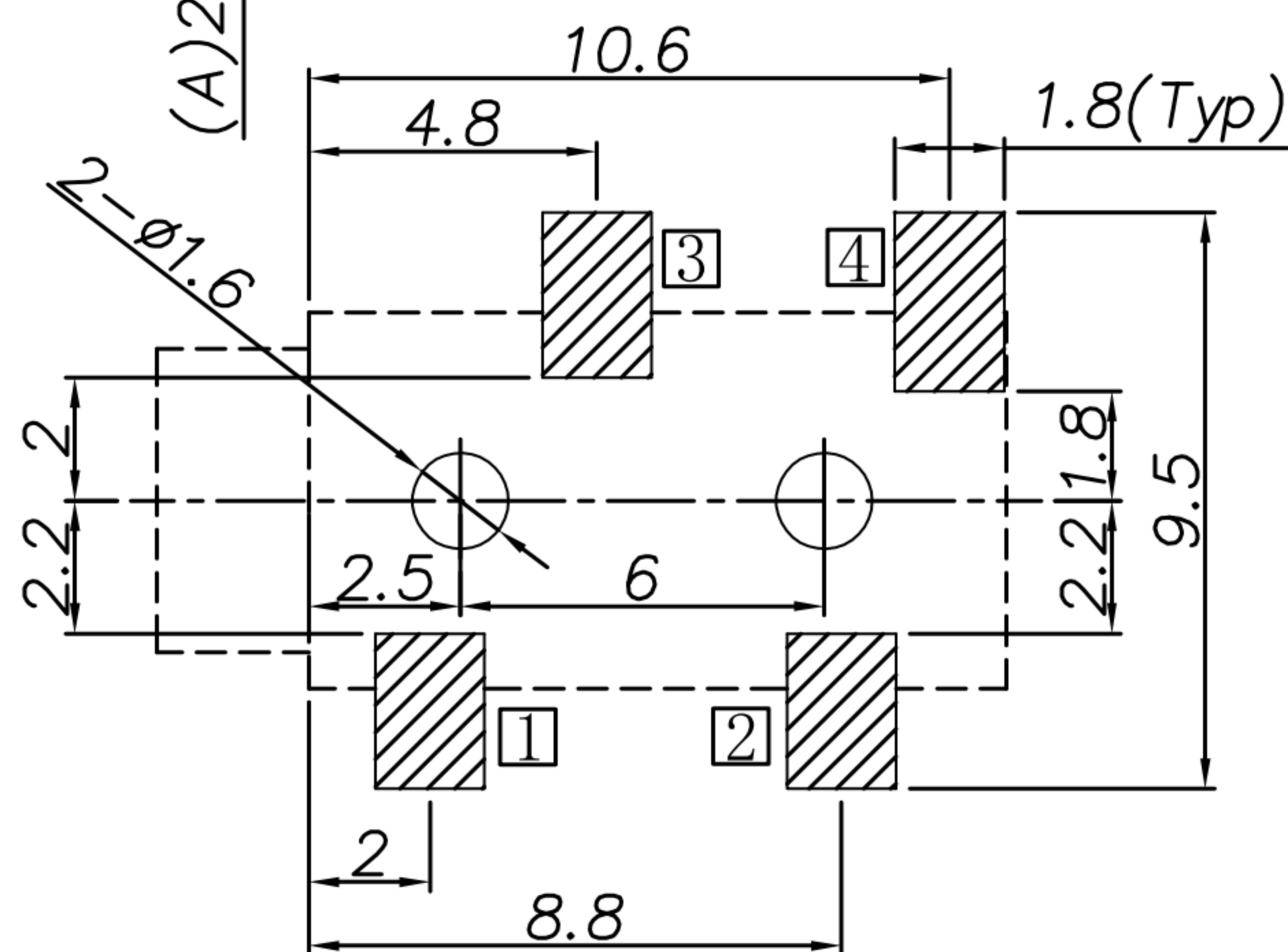
P. C. B Layout (Copper-sided view)
